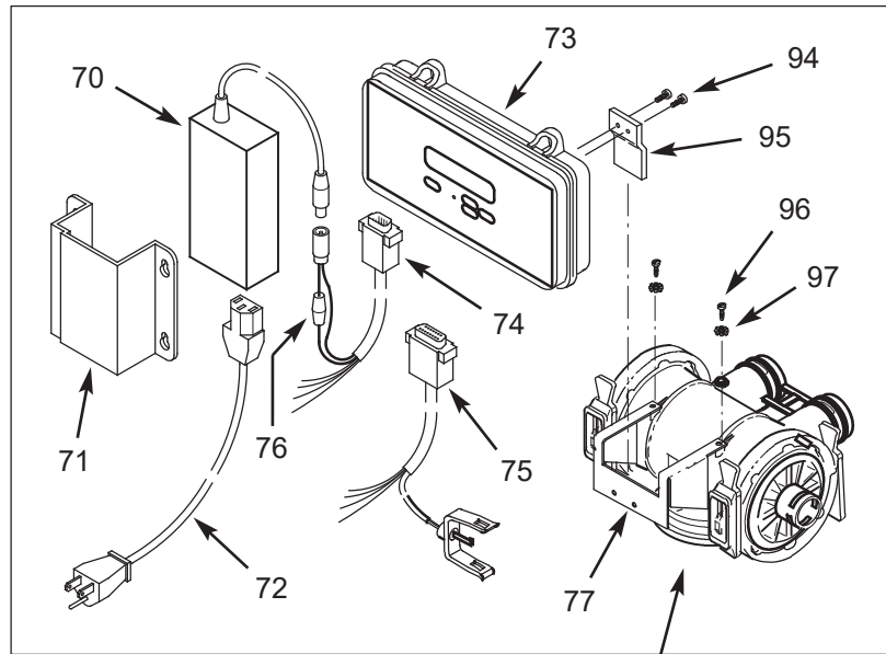
1" Dual Disc Valve Assembly See Pages 10 & 11 for parts
