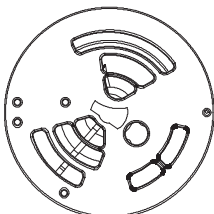
Rotor & Disc, Single Tank, Filters & Softeners EWS 471 & 071
