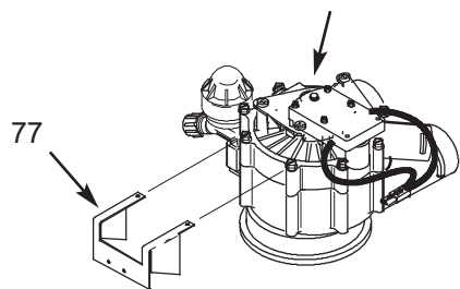
1" Single Disc Valve Assembly See Pages 8 & 9 for parts
