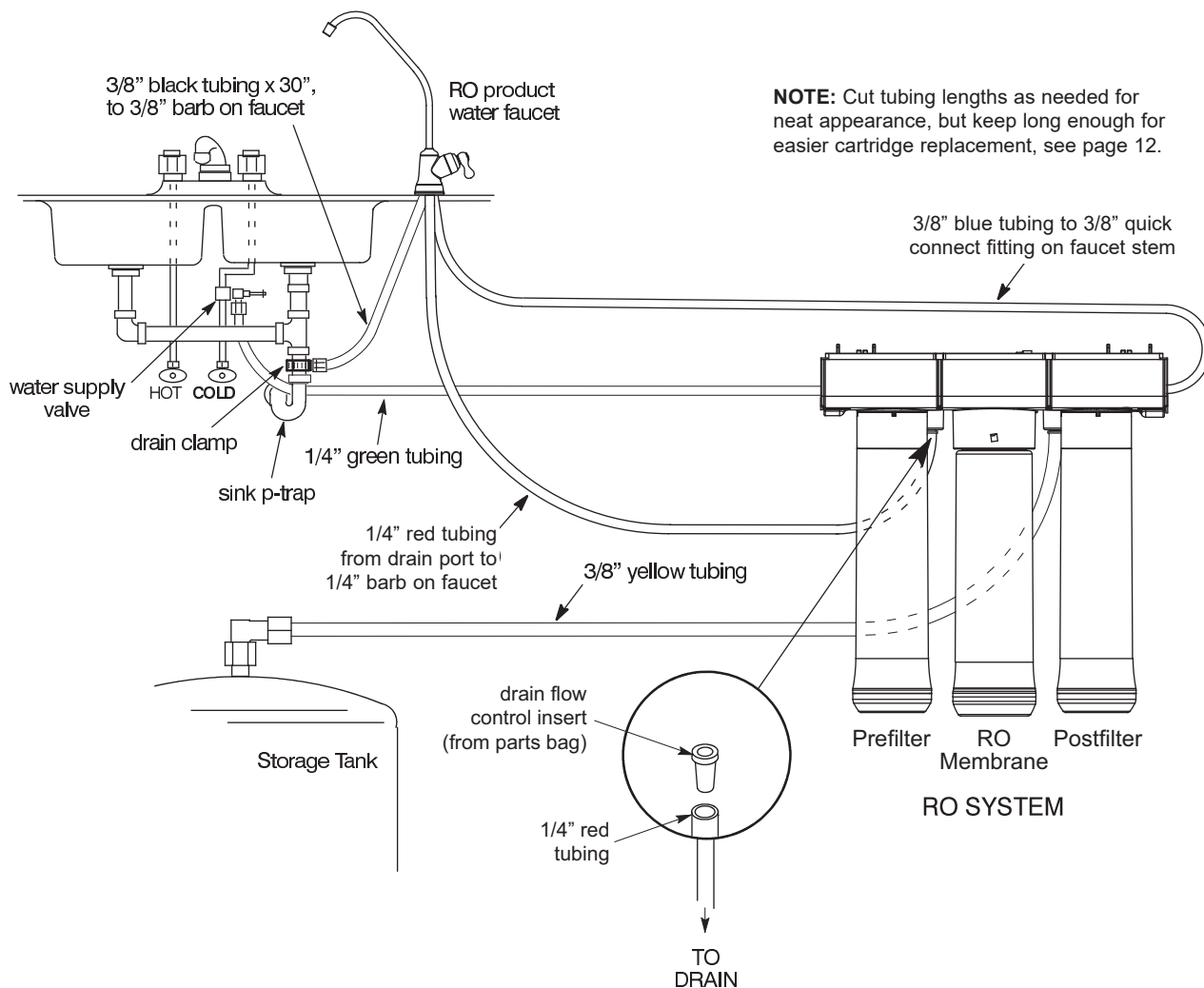
FIGURE 5 - TYPICAL INSTALLATION
