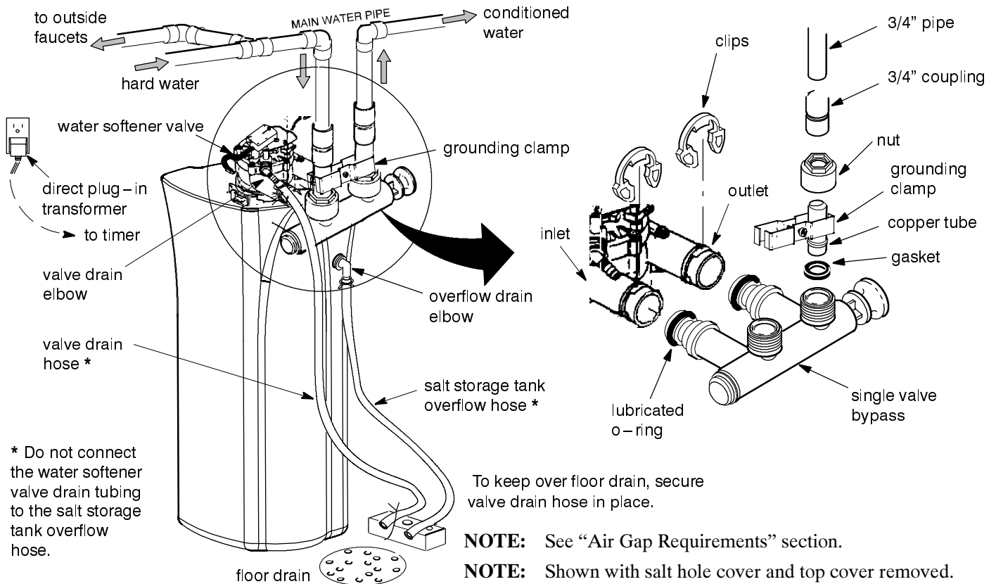
Figure 5 (typical installation)
